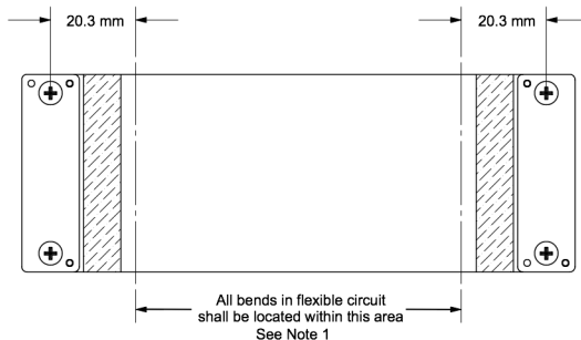
Figure 1-7. Flex Cable Diagram
