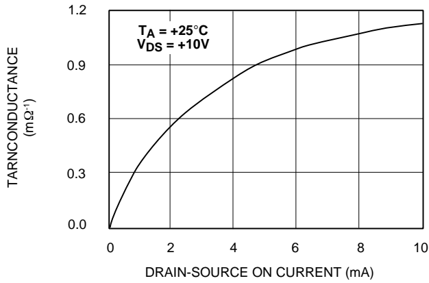
TRANCONDUCTANCE vs. DRAIN-SOURCE ON CURRENT
