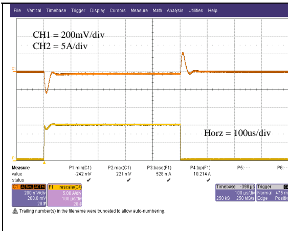
Vo=1.8V Typical output voltage transient response to load step from 25% to 75% of full load with output current slew rate of 10A/uS. (Cext = 4x47uF ceramic capacitor)
