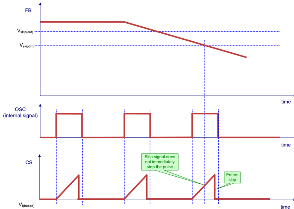
Figure 62. Technique Preventing Short Pulses in Skip Mode
