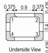
Underside View
