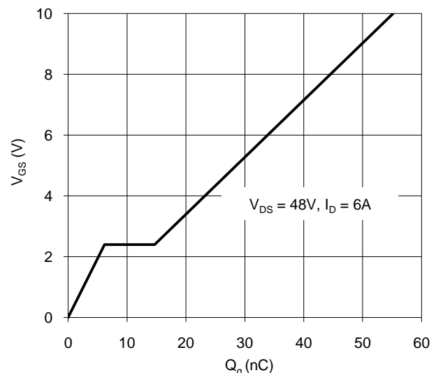
Figure 12. Gate Charge
