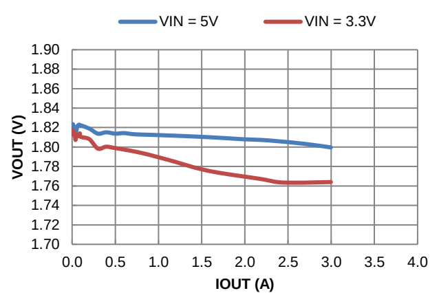
Figure 13. Load Regulation
