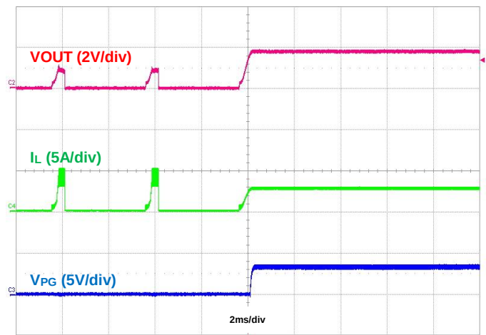
Figure 40. Output Short Recovery, IOUT = 3A
