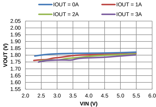
Figure 23. Line Regulation
