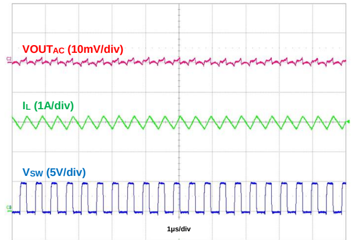
Figure 17. Output Voltage Ripple, I_{OUT} = 3\text{A}
