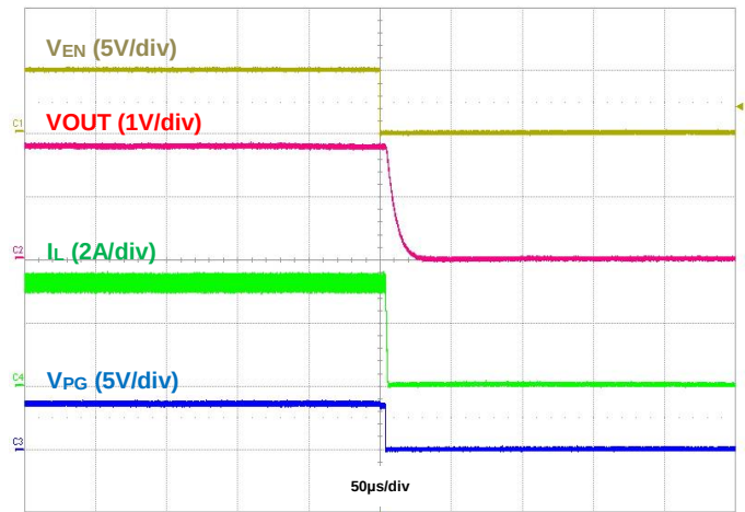
Figure 38. Shutdown Using EN, IOUT = 3A
