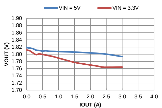
Figure 24. Load Regulation
