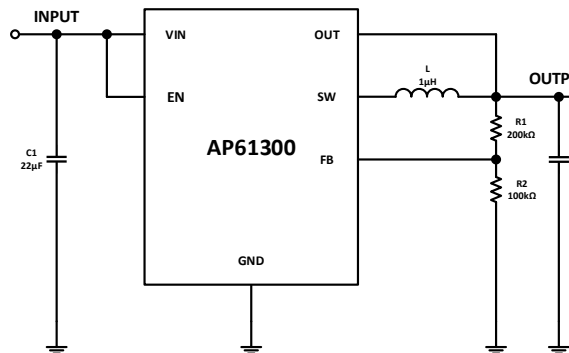
Figure 1. Typical AP61300 Application Circuit
