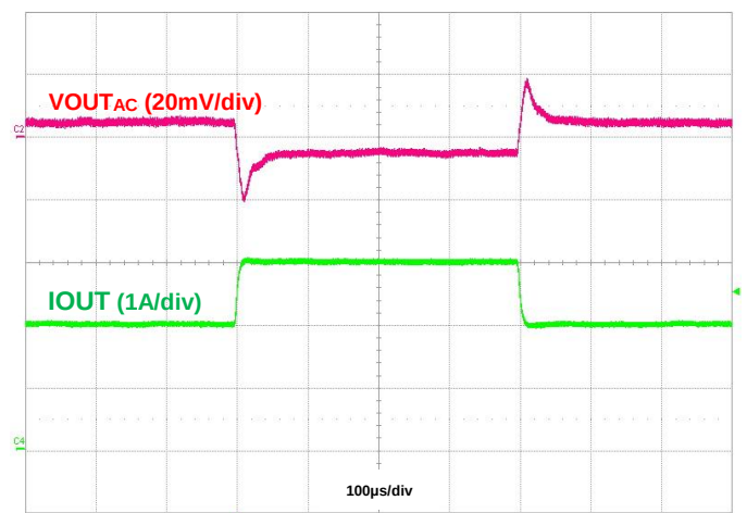
Figure 19. Load Transient, I_{OUT} = 2\text{A} to 3\text{A} to 2\text{A}
