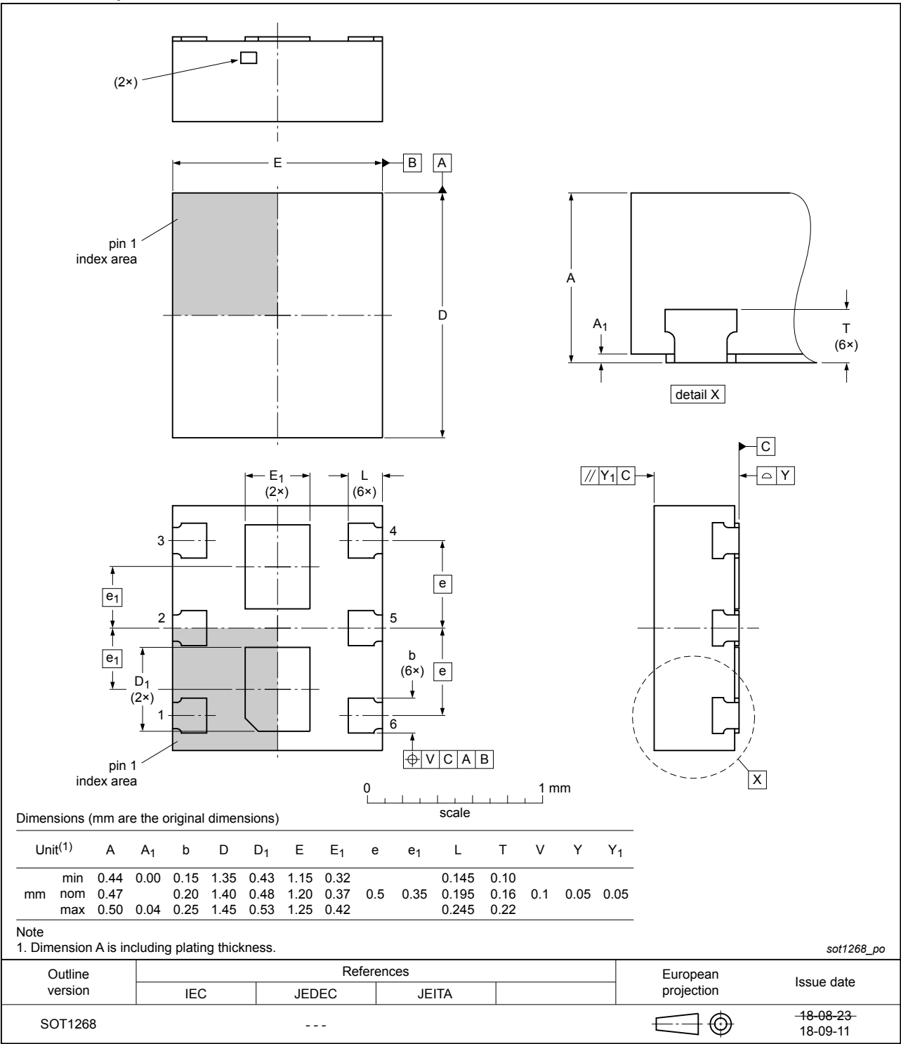
Fig. 10. Package outline DFN1412-6 (SOT1268)
