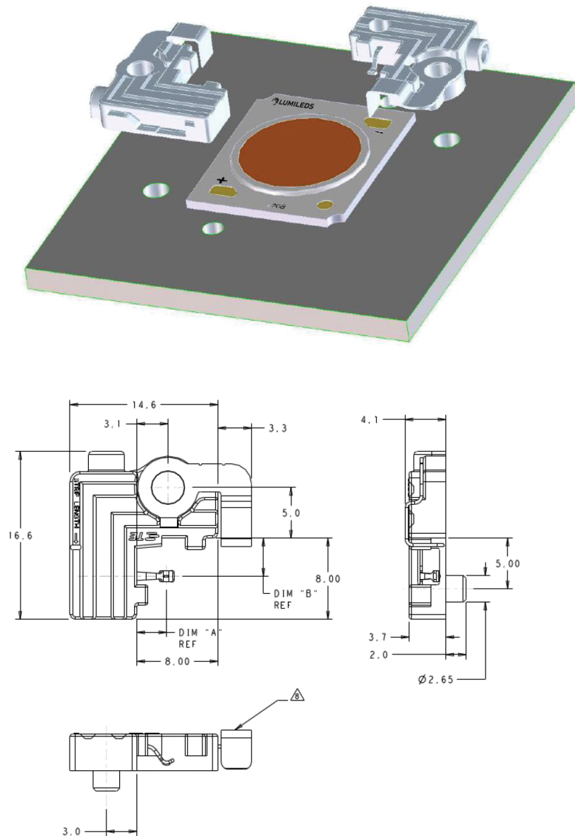
Figure 2. Reference dimensions for TE 2-2154857-2, a scalable solder-less connector for mounting LUXEON CoB emitters. See TE Application Specification 114-32043 for detailed mounting instructions.
