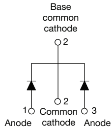
VS-20CTQ...S-M3
