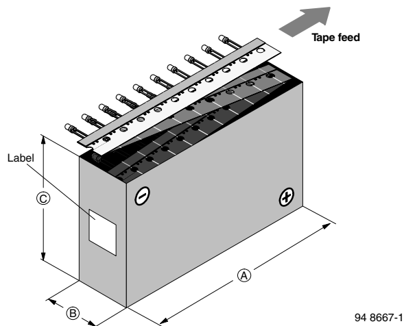
Fig. 12 - Tape Direction
