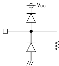
Pin 10 (REF)
