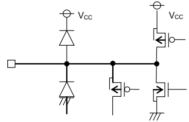
Pin 9 (SS/TRACK)
