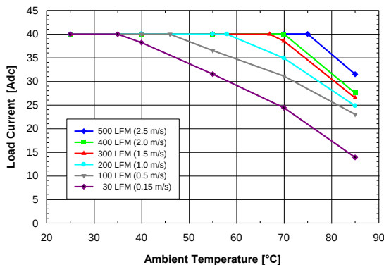
Figure 1. Available output current vs. ambient air temperature and airflow rates for converter DP8140G mounted horizontally with air flowing from input to output, Vin = 12 V, Vout = 3.3 V, and Fsw = 500 KHz
