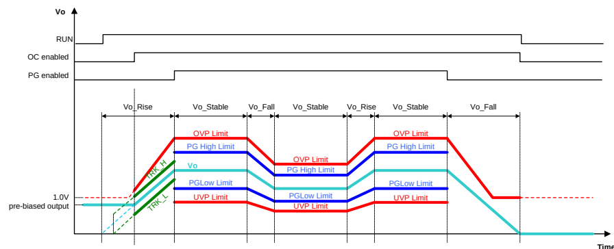
Figure 26. Protection Enable Conditions
