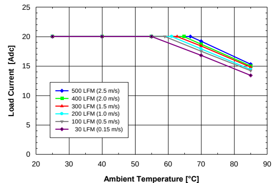
Figure 2. Available output current vs. ambient air temperature and airflow rates for converter DP8140G mounted horizontally with air flowing from input to output, MOSFET temperature ≤ 120°C, Vin = 12 V, Vout = 5 V, and Fsw = 500 KHz
