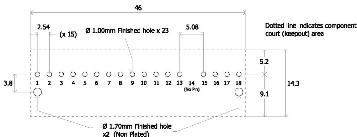
Figure 53. Pinout Diagram (Bottom View)
