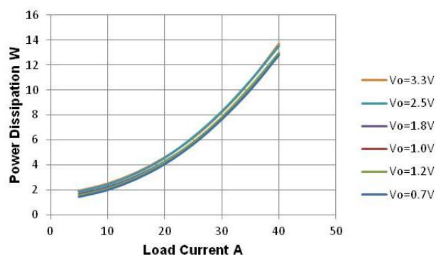
Figure 4. Dissipation vs Load, V_{in}=8V , F_{sw}=500kHz
