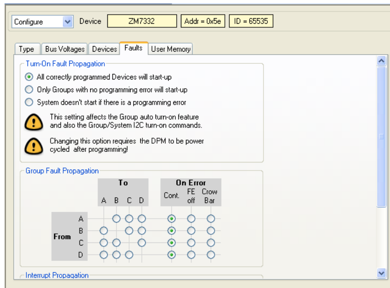
Figure 30. Protection Configuration Register PC3
