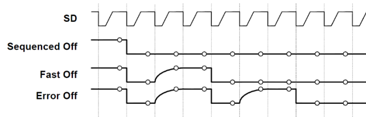
Figure 36. OK Severity Encoding Waveforms
