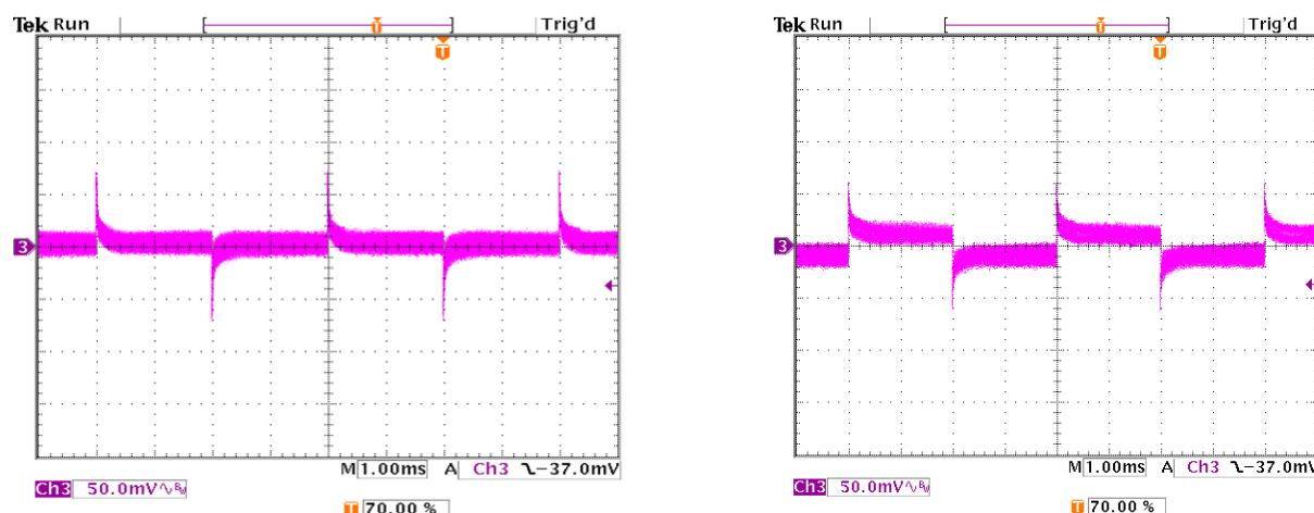
Figure 45. Transient Response with Regulation set to 0.55mV/A
