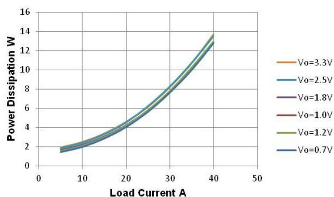
Figure 2. Dissipation vs Load, V_{in}=12V , F_{sw}=500kHz
