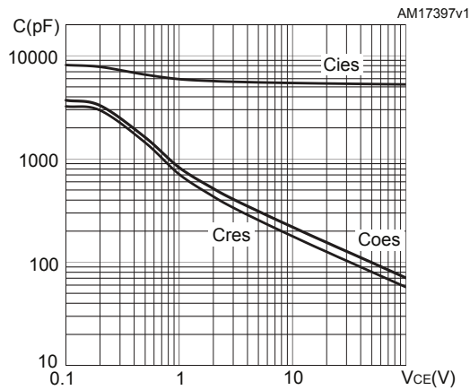
Figure 17. Capacitance variations
