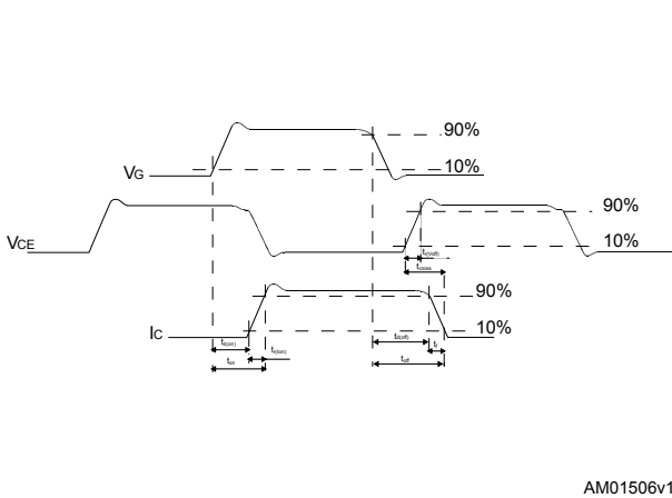
Figure 35. Switching waveform
