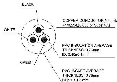
Wire cross section
