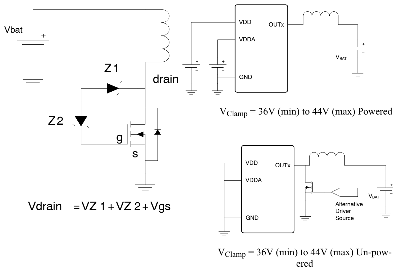
Figure 22. Output Clamp
