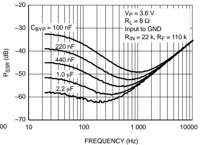
Figure 13. P_{SRR} versus Frequency and C_{BYP} @ V_P = 3.6 \text{ V} , A_V = 10
