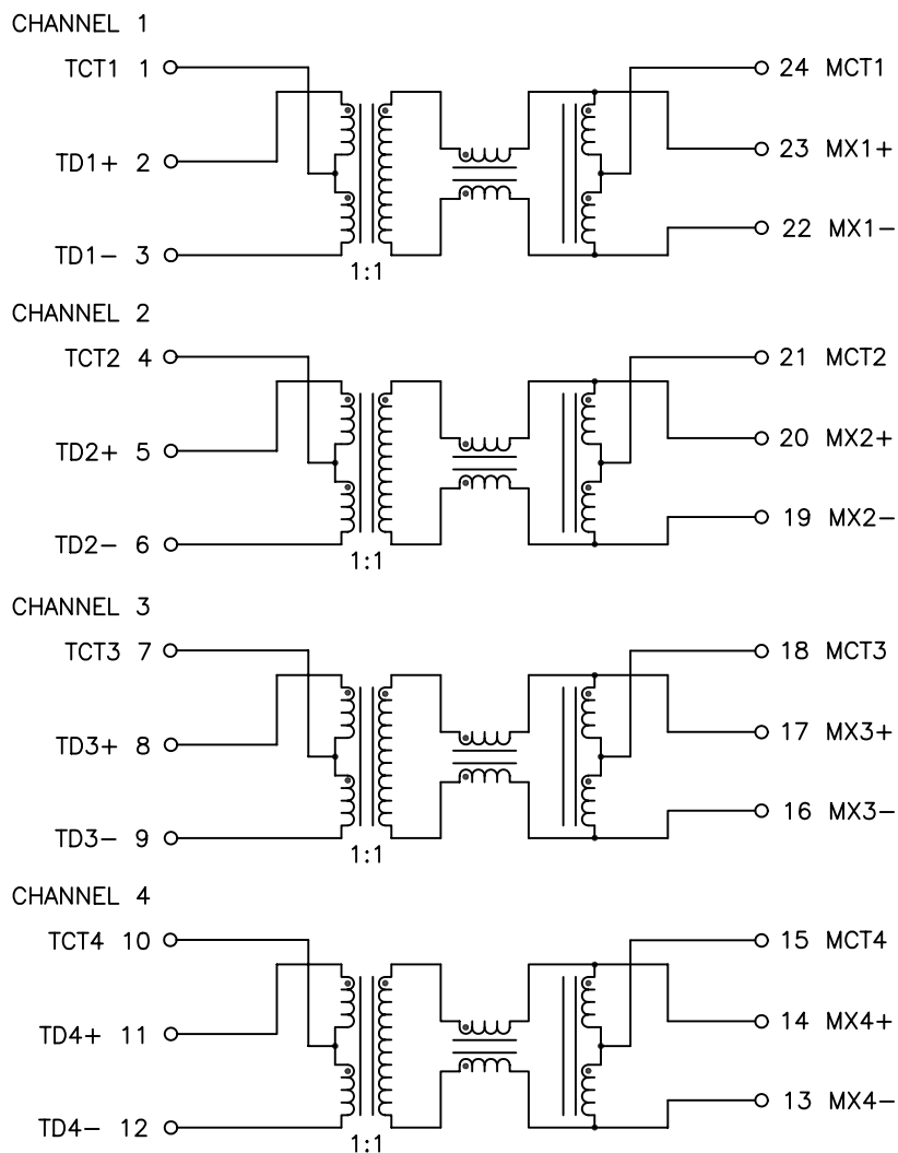
SCHEMATIC
