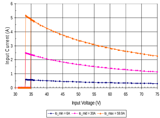
Typical Input Current vs. Input Voltage Characteristics
