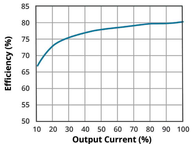
EFFICIENCY VS OUTPUT LOAD AE15-EW-S12-DIN
