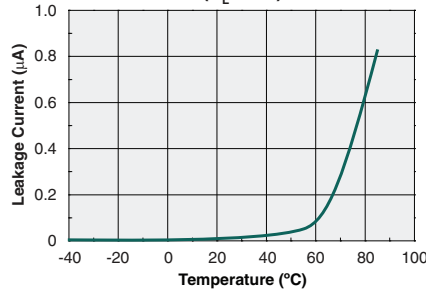
Leakage Current vs. Temperature Across Pins 5&6, 7&8 ( V_L=60V )
