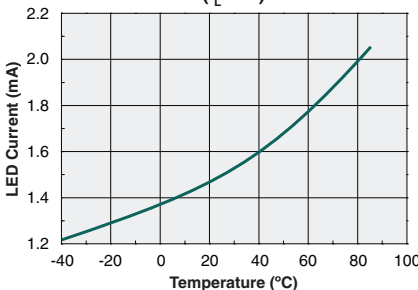
Typical I_F for Switch Operation ( I_L=1\text{A} )
