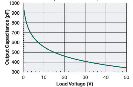
Output Capacitance vs. Load Voltage ( I_F=0mA, f=1MHz )
