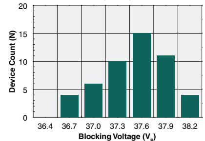
Blocking Voltage Distribution (N=50)
