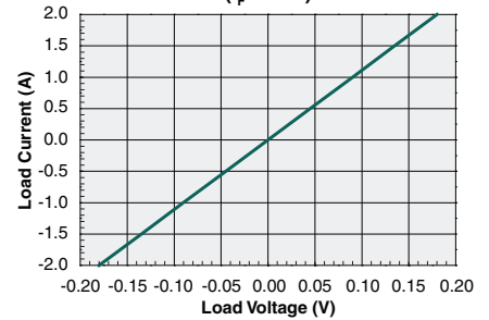
Typical Load Current vs. Load Voltage ( I_F=2mA )
