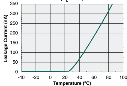
Typical Leakage vs. Temperature Measured Across Pins 4&6 ( V_L=30V )
