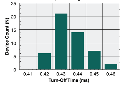
Typical Turn-Off Time Distribution (N=50, I_F=5\text{mA} , I_L=120\text{mA} )
