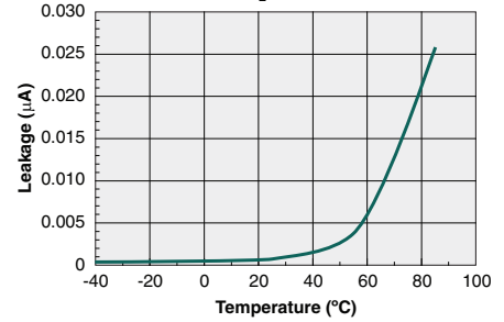
Typical Leakage vs. Temperature Measured Across Pins 5&6, 7&8 ( V_L=400V )
