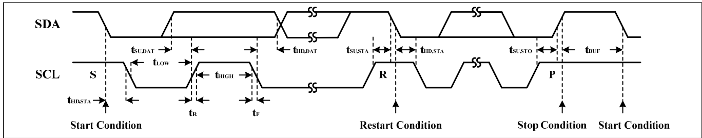
Figure 4 Interface Timing
