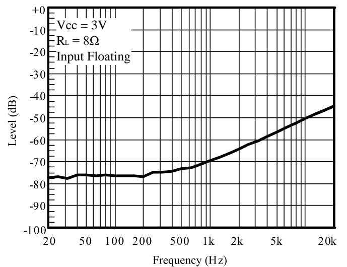
Figure 13 PSRR vs. Frequency
