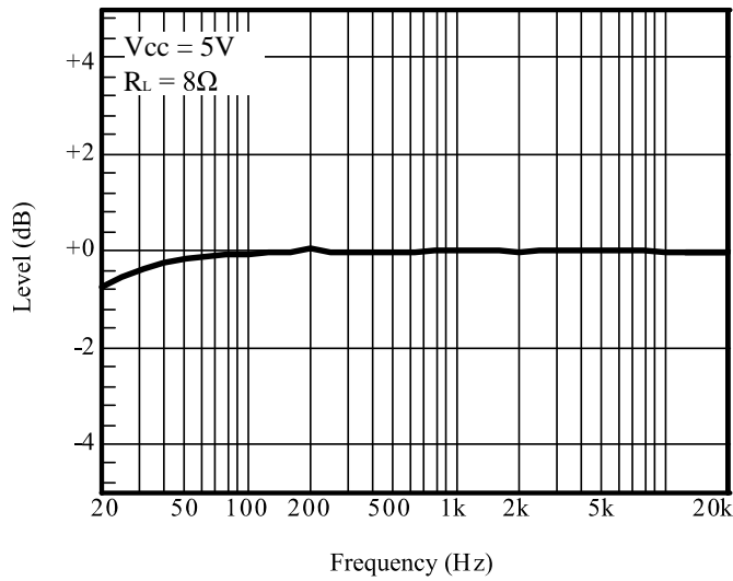
Figure 14 Frequency Response
