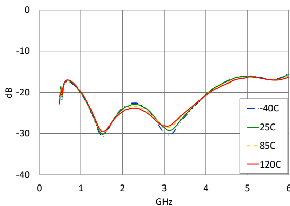
TX Return Loss in TX ON state
