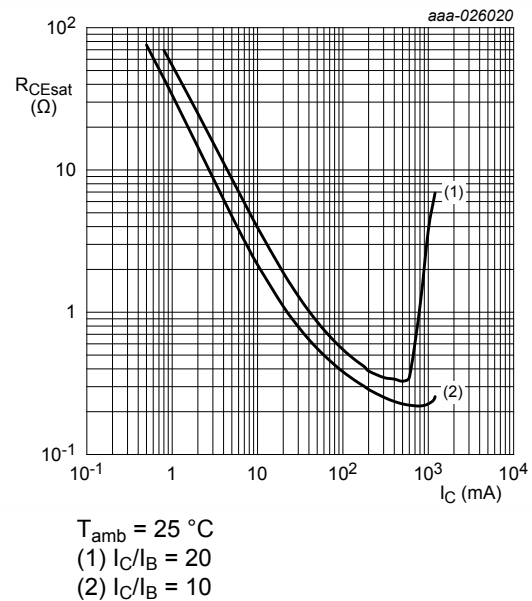
Fig. 10. Collector-emitter saturation resistance as a function of collector current; typical values
