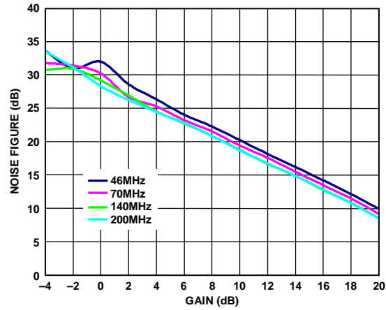
Figure 20. NF vs. Gain at 46 MHz, 70 MHz, 140 MHz, and 200 MHz
