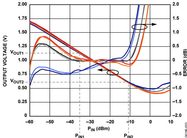
Figure 60. Transfer Function at 2.2 GHz with Calibration Points
