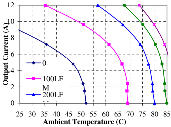
Figure 8. HD20ZGB Derating Curves
