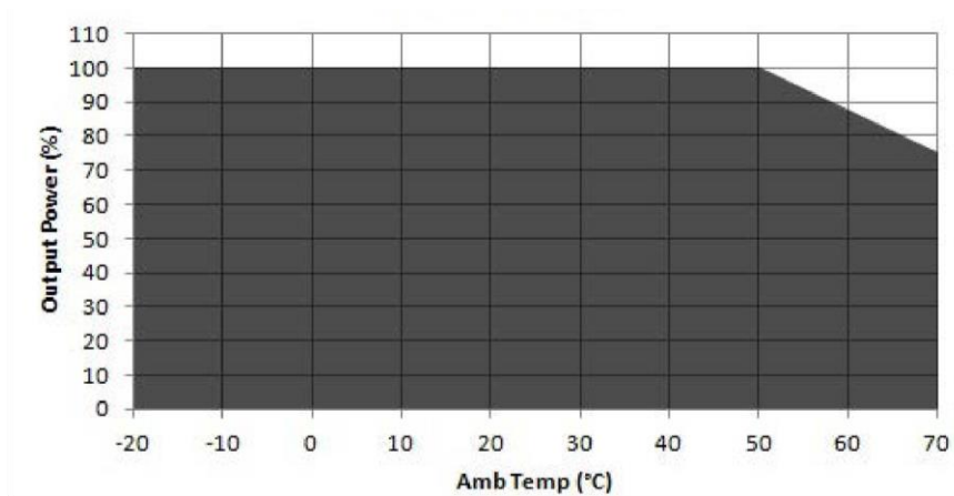
Figure 1. Derating Curve
