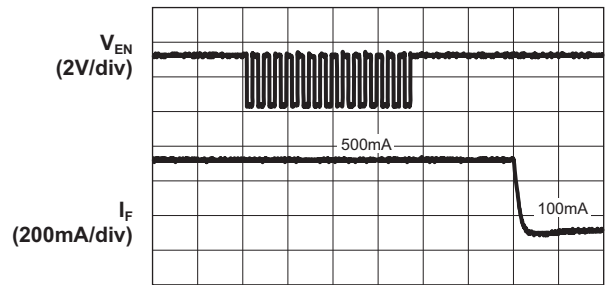
LED Current Transient by EN/SET
