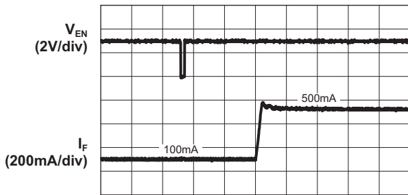
LED Current Transient by EN/SET
