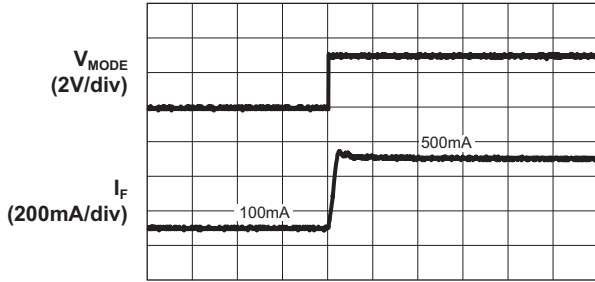
LED Current Transient by MODE Change
