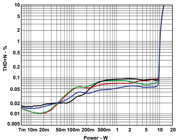
Figure 4. THD+N vs Power (SE – 3 Ω)
