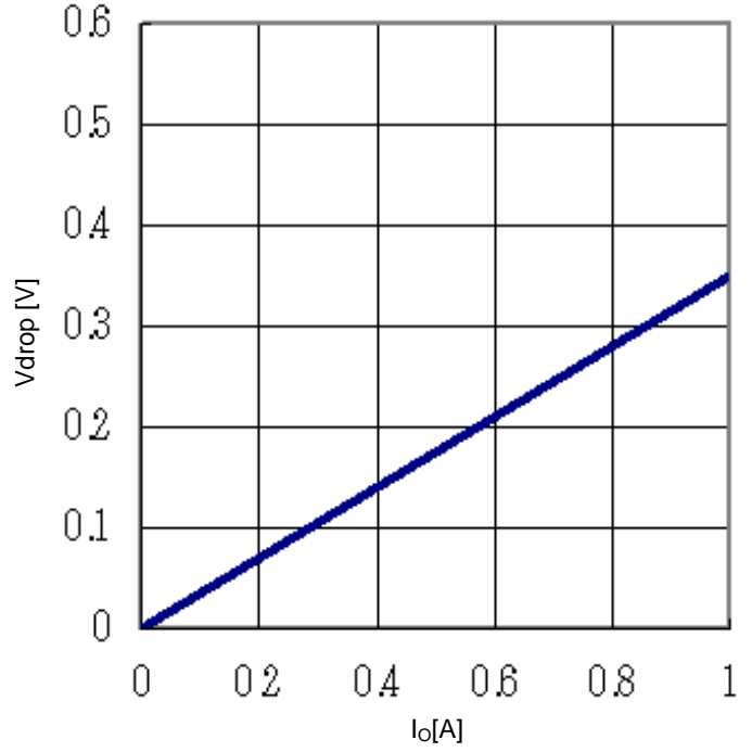
Fig.23 Minimum dropout Voltage 4 (V CC =8V、Ta=25°C)
