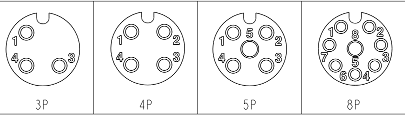
Pin Assignments Front View
