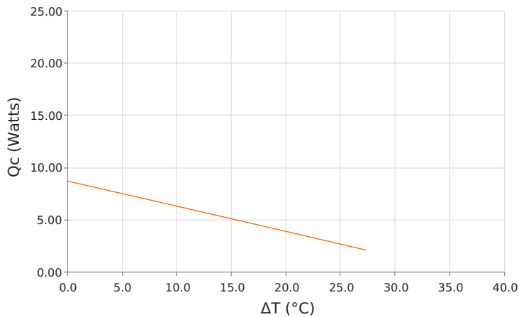
Heat Pumped at Cold Side ( Q_c ) T_{hot} = 85^\circ\text{C} | Current = 7.5 Amps
