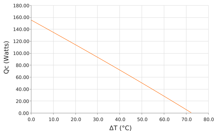
Heat Pumped at Cold Side ( Q_c ) T_{hot} = 27\text{ }^{\circ}\text{C} | Current = 10.4 Amps
