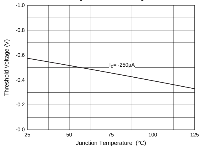
Fig. 6 - Threshold Voltage
