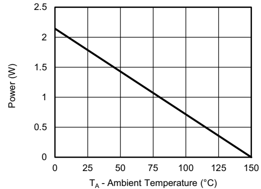
Power, Junction-to-Ambient
