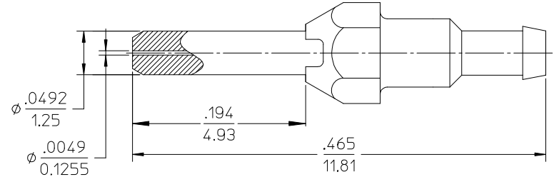
SNAP MATE PLUG, METAL BODY (ZIRCONIA CERAMIC FERRULE)
