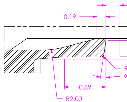
DETAIL 'D' SCALE 20:1 (ALL DIMS TYP)
