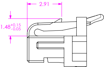
PRE-LOAD VIEW
