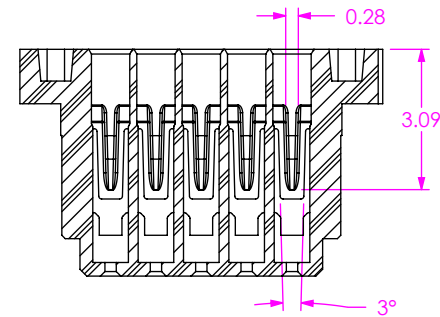
SECTION "E"- "E" (ALL DIMS TYP)
