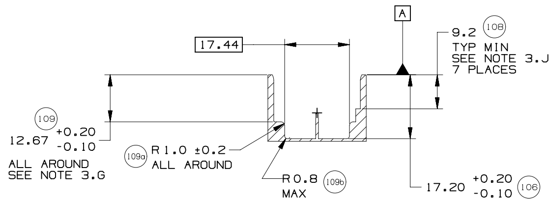
SECTION R-R
