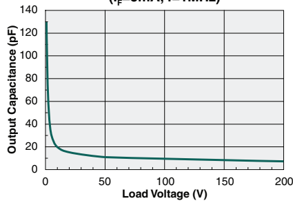
Output Capacitance vs. Load Voltage ( I_F=5\text{mA} , f=1\text{MHz} )
