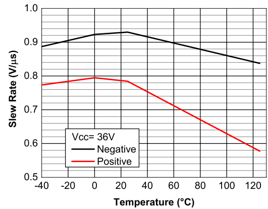
Figure 16. Slew rate behavior vs. temperature at V_{CC} = 36\text{ V}
