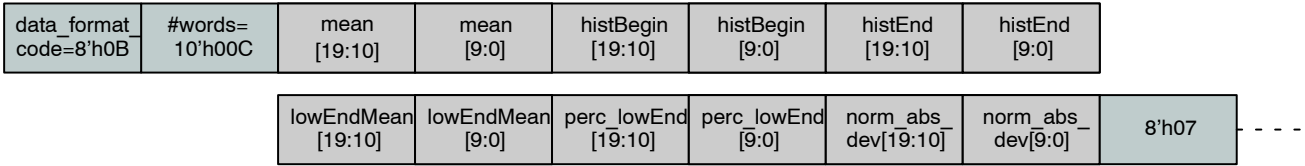
Figure 36. Format of Embedded Statistics Output within a Frame
