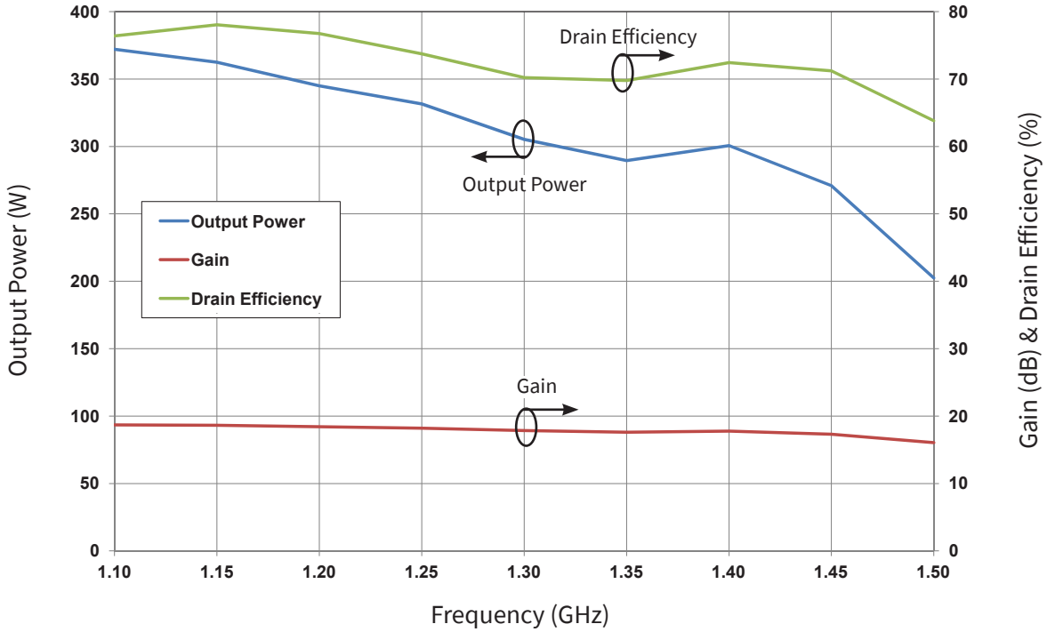
CGHV14250 Typical RF Results V_{DD} = 50\text{ V}, I_{DQ} = 500\text{ mA}, P_{IN} = 37\text{ dBm} T_{case} = 85^\circ\text{C}, \text{Pulse Width} = 500\ \mu\text{s}, \text{Duty Cycle} = 10\%
