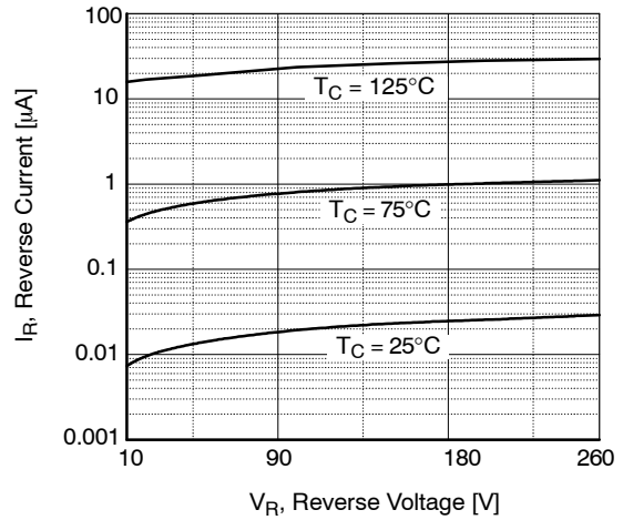
Figure 4. Typical Reverse Current vs. Reverse Voltage
