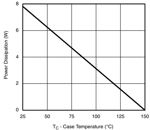
Power Derating
