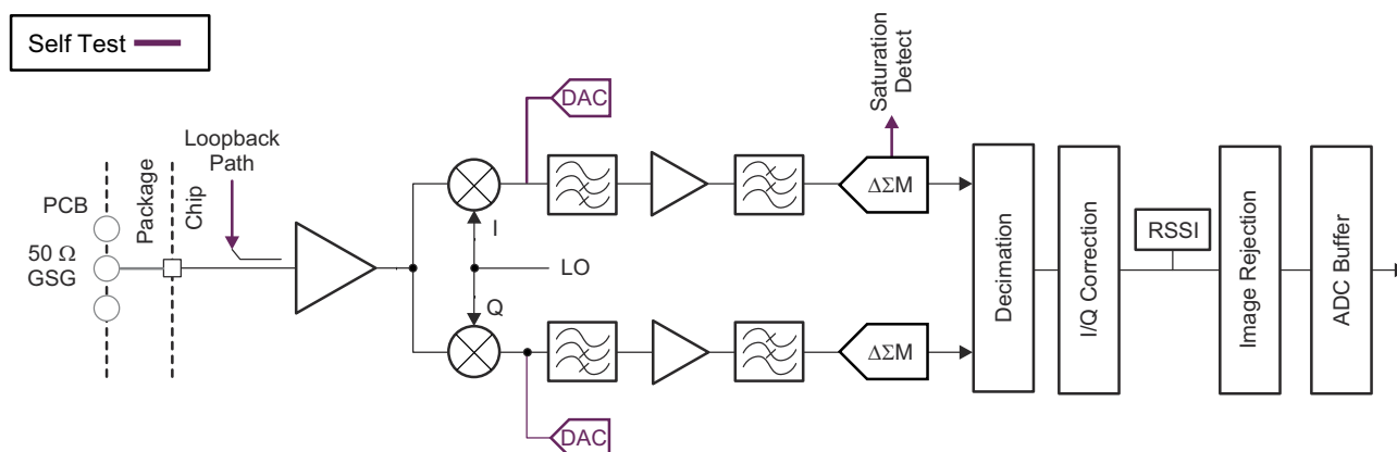
Figure 9-3. Receive Subsystem (Per Channel)
