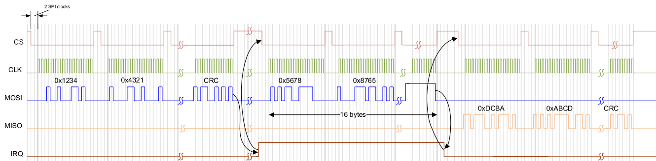
Figure 8-6. SPI Communication
