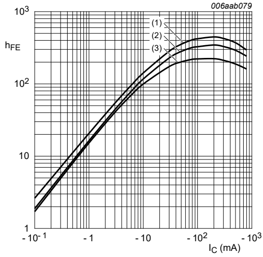
V_{CE} = -5 V (1) T_{amb} = 100^\circ C (2) T_{amb} = 25^\circ C (3) T_{amb} = -40^\circ C
